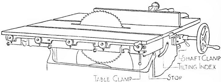
FIG. 159. TABLE ADJUSTMENTS.
